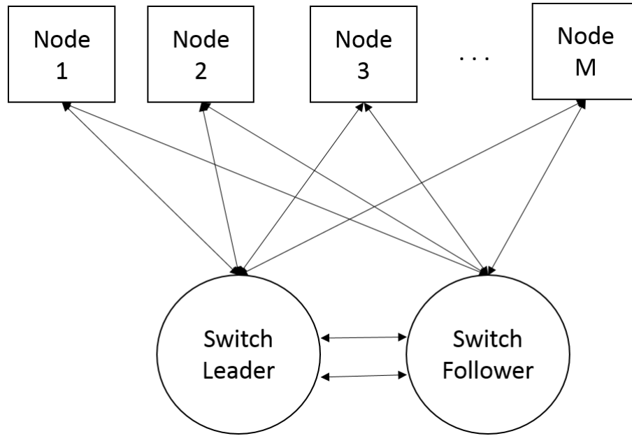
FIGURE 3.4: FTTRS architecture
