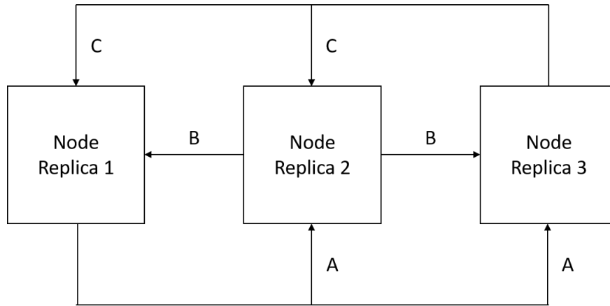
FIGURE 5.8: CC-vector exchange between 3 node replicas
