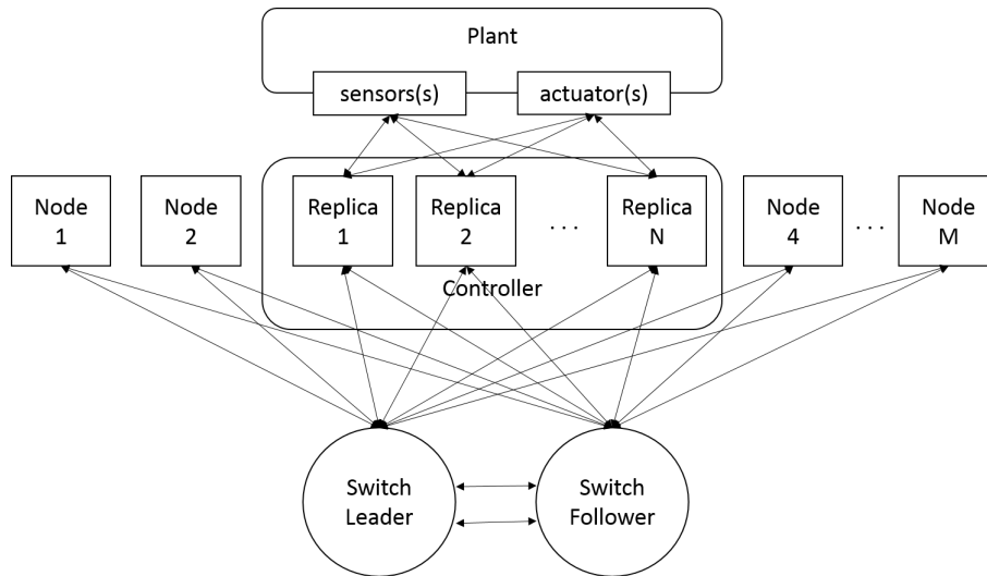
FIGURE 6.1: Control Application Architecture
