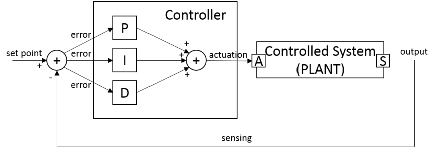
FIGURE 6.3: PID controller
